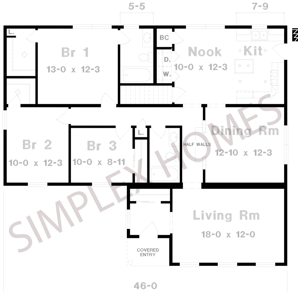
WASHBURN II FLOOR PLAN 26/38 X 46 1500 SQ FT
