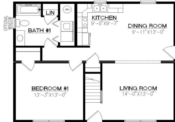
First Floor (w/ Crawl Space)
