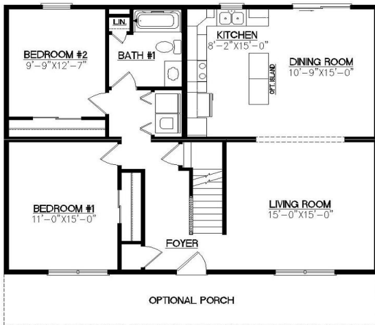
First Floor (w/ Basement)
