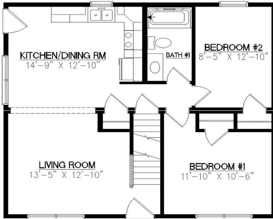
First Floor (w/ Basement)
