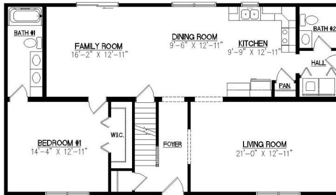
First Floor (w/ Basement)
