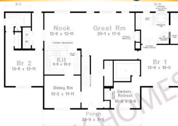
WILLIAMSBURG CAPE FIRST FLOOR PLAN 64-0 X 41-5 2250 Sq. Ft.
