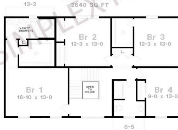
FITCHBURG II 27-6 X 48 SECOND FLOOR PLAN
