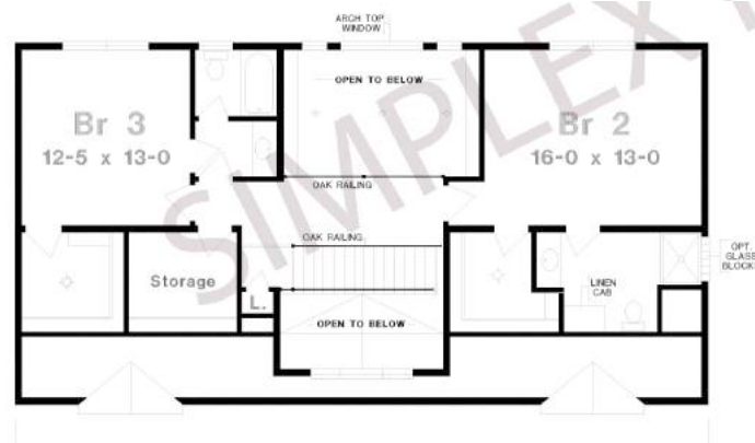
2ND. FL. FLOOR PLAN - CAMBRIDGE II
